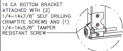
DETAIL D
