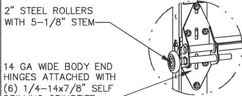
DETAIL B
